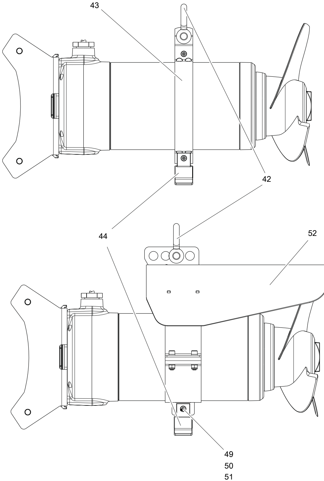
Figure 1: Lifting device and vortex protection shield
